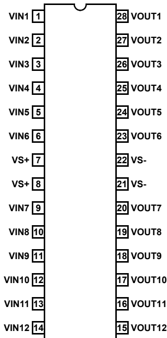
EL5423 (28-PIN TSSOP) TOP VIEW
